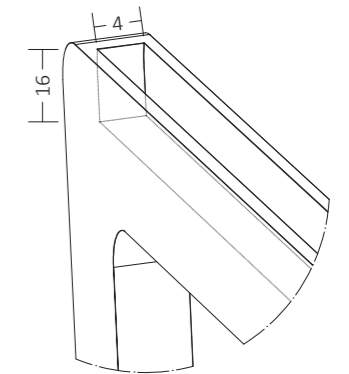
DETAIL IV SCALE 1:1 PLEXIGLASS CAVITY
