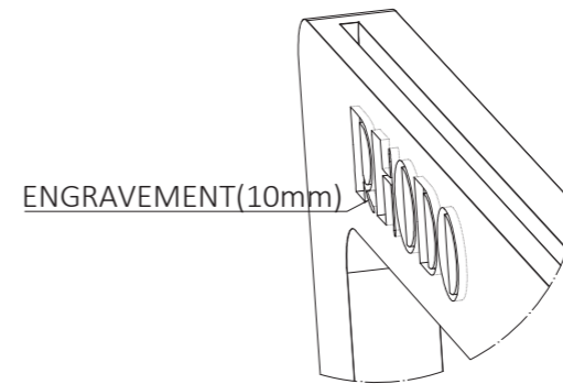
DETAIL III SCALE 1:1 LOGO LASER ENGRAVE
