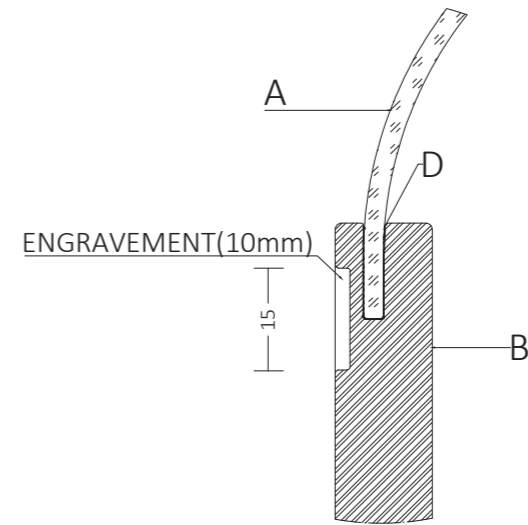
DETAIL I SCALE 1:1 I-I' PARTIAL SECTION
