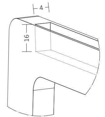
DETAIL III SCALE 1:1 PLEXIGLASS CAVITY
