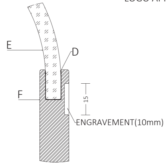
DETAIL II SCALE 1:1 I-I' PARTIAL SECTION
